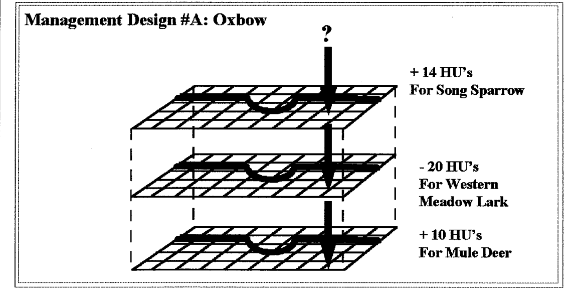
Figure 4. 3 - Dimensional Matrix
