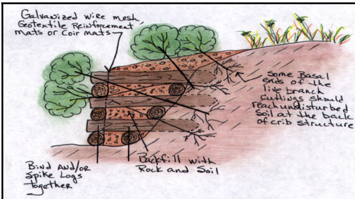
Live Cribwall or Typical Log Cribbing adapted from "Erosion Draw"
