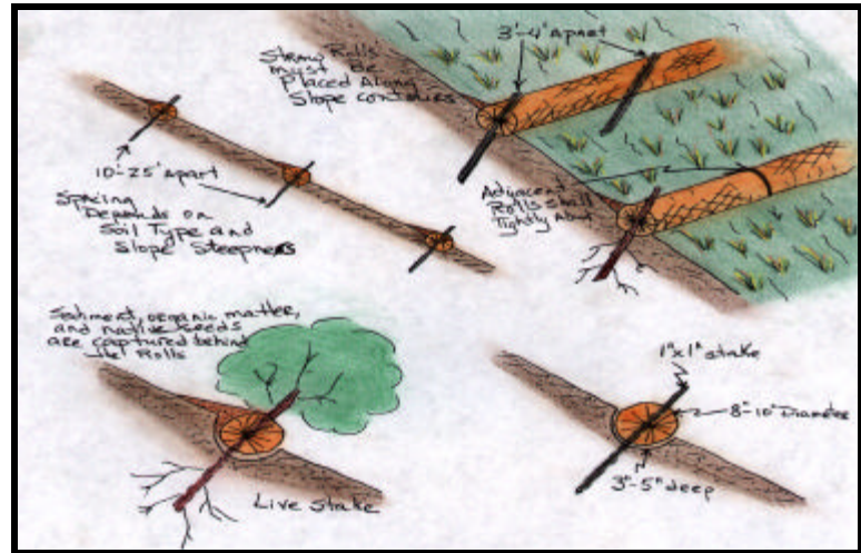
Straw Rolls adapted from "Erosion Draw"
