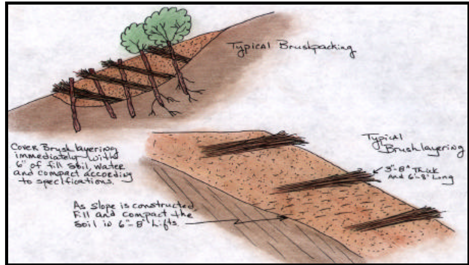
Brushlayer and Brushpacking adapted from "Erosion Draw"
