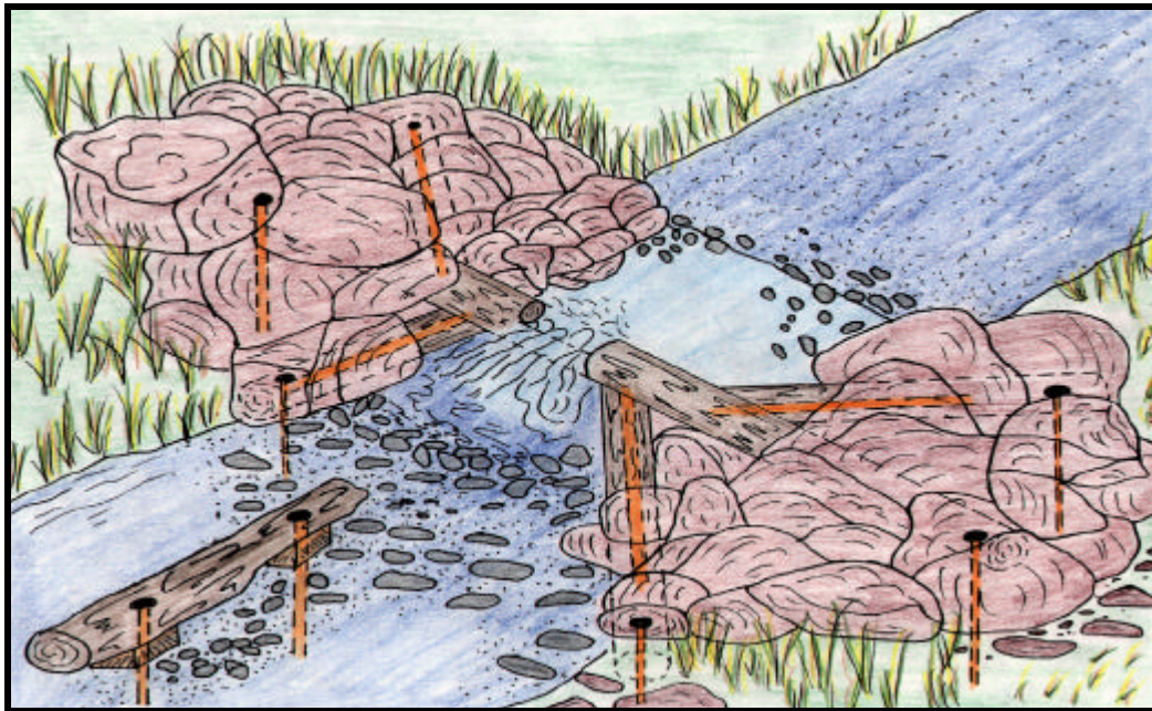
K-Dam and Whole Log Cover adapted from "Trout Stream Therapy"
