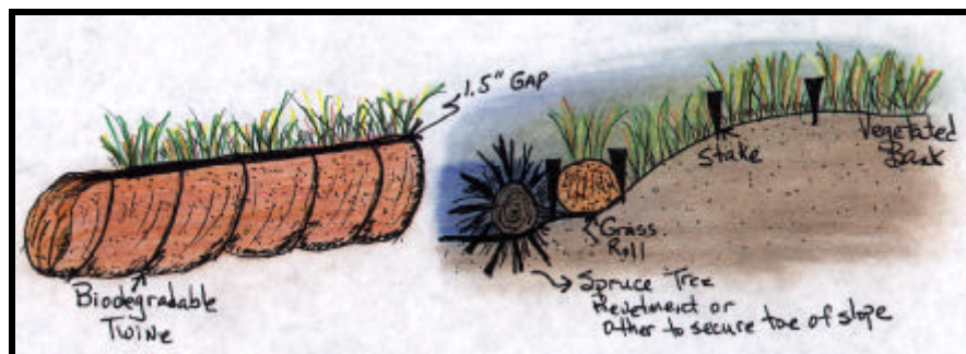
Grass Rolls
