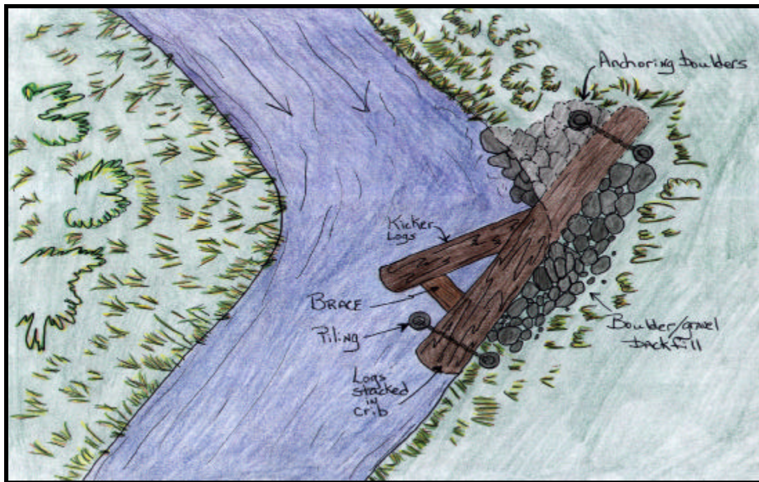
Log Crib Bank Protection adapted from "Applied River Morphology"
