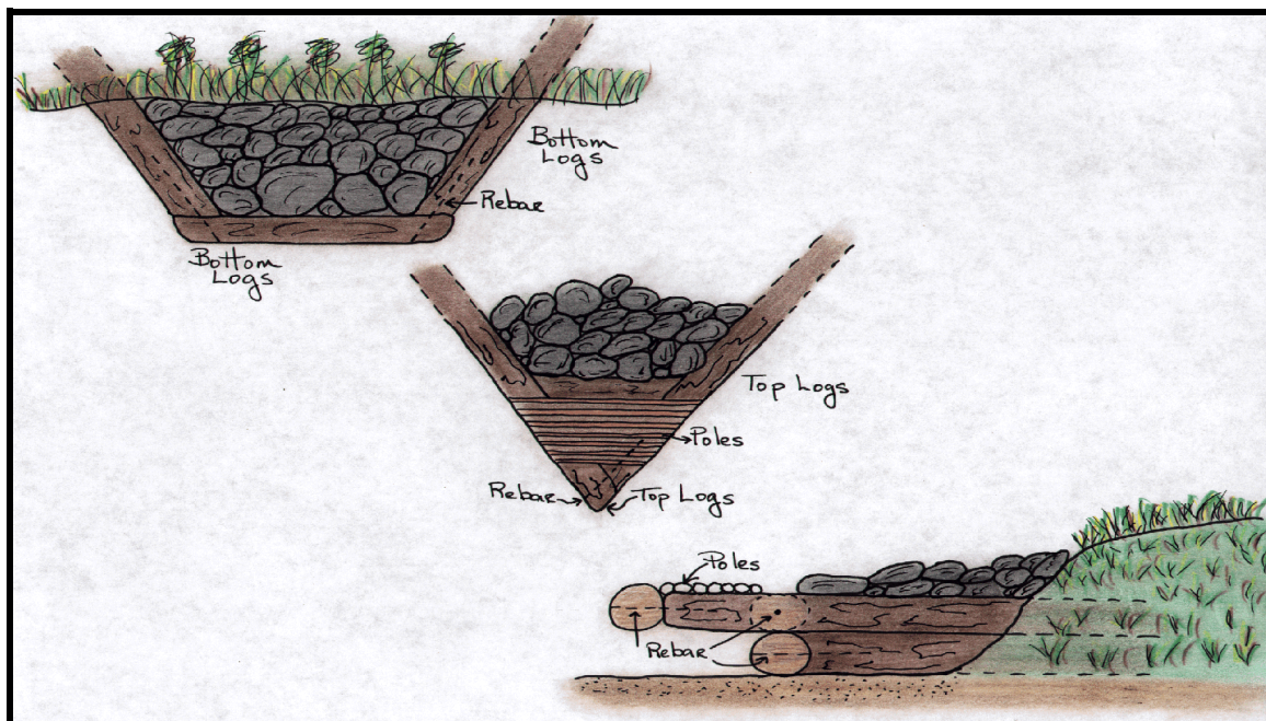
Tip Deflector adapted from the Forest Service
