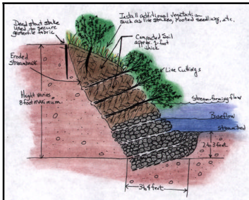
Vegetated Geogrids adapted from U.S. Department of Agriculture
