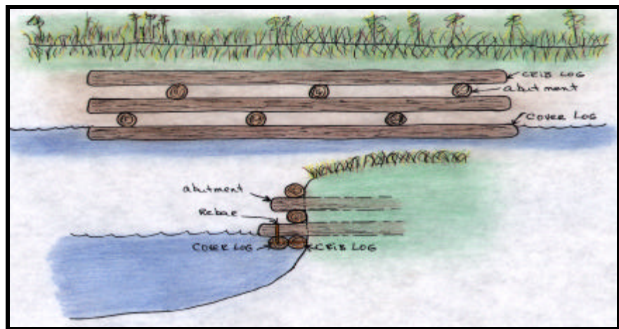
Bank Crib with Cover Log adapted from the Forest Service - USDA
