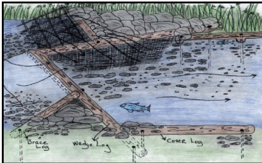
Wedge Dam
