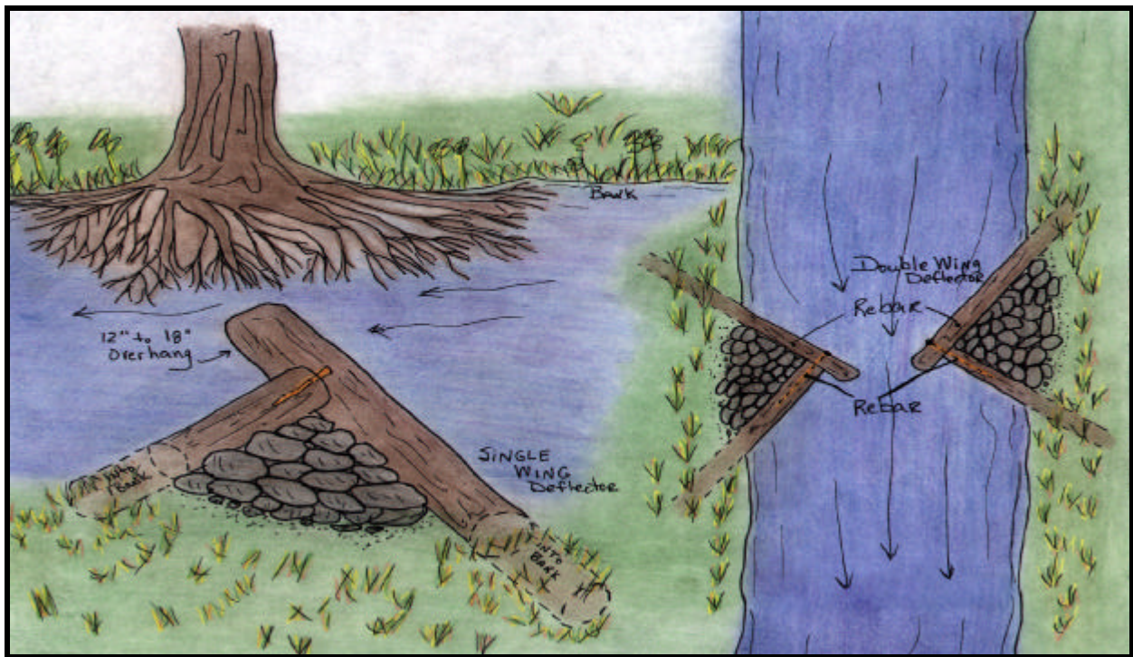
Single- and Double-Wing Deflector adapted from the Forest Service
