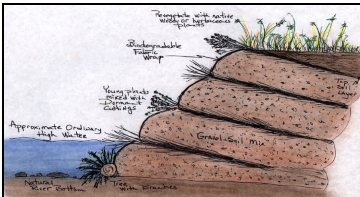
Hedge-Brush Layering adapted from the State of Alaska
