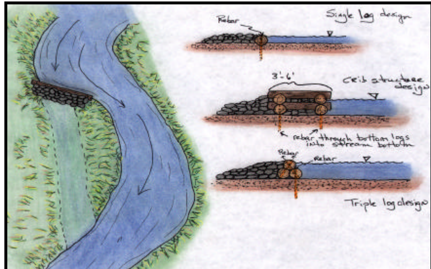
Channel Block adapted from the Forest Service
