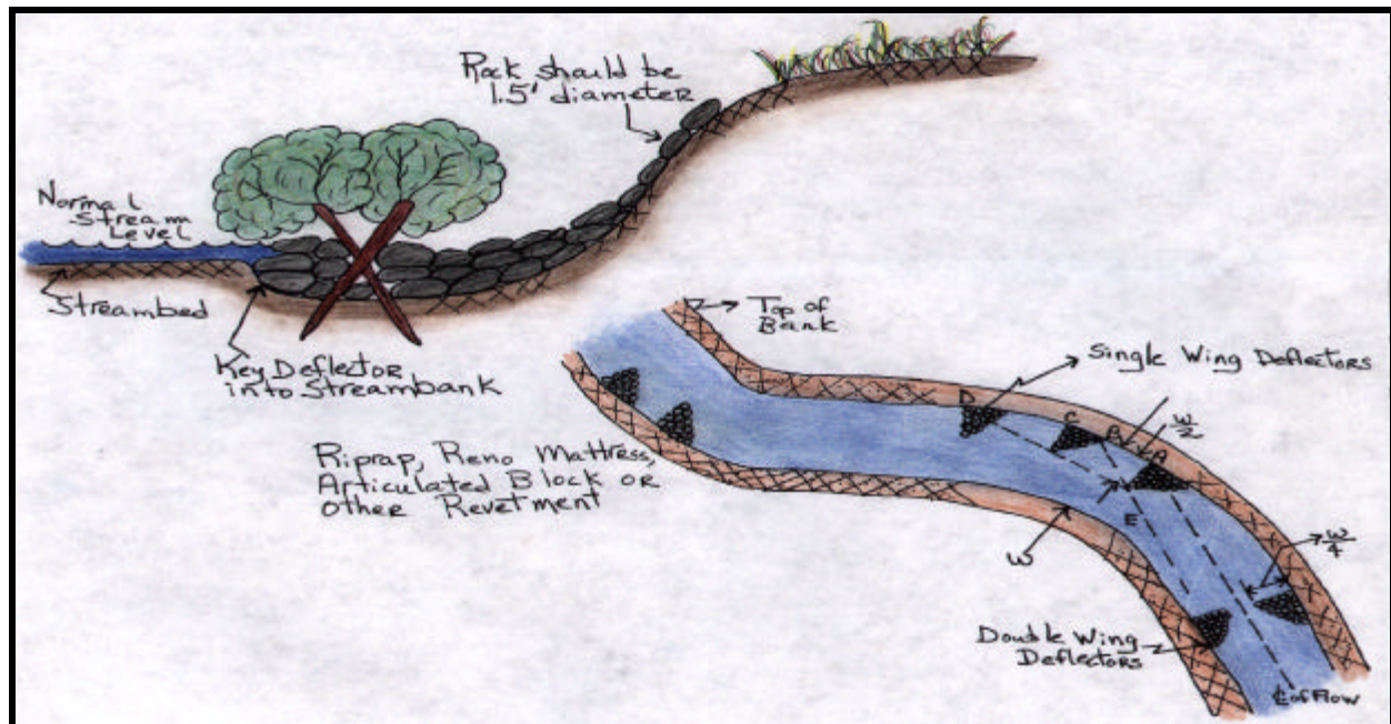
Rock Deflectors
