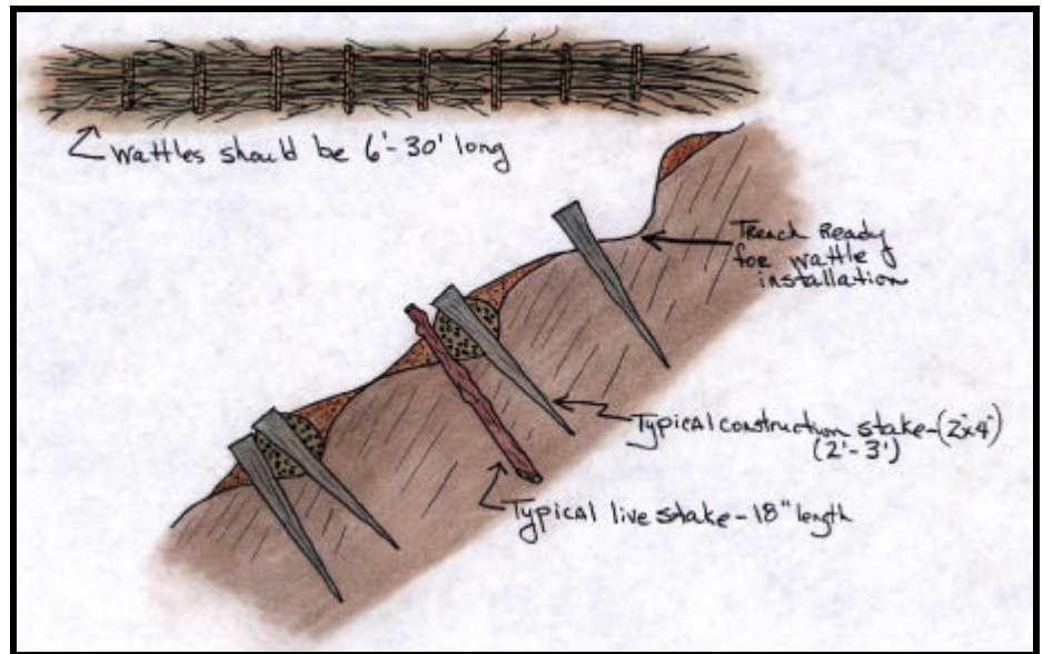
Live Fascines or Wattlings adapted from "Erosion Draw"
