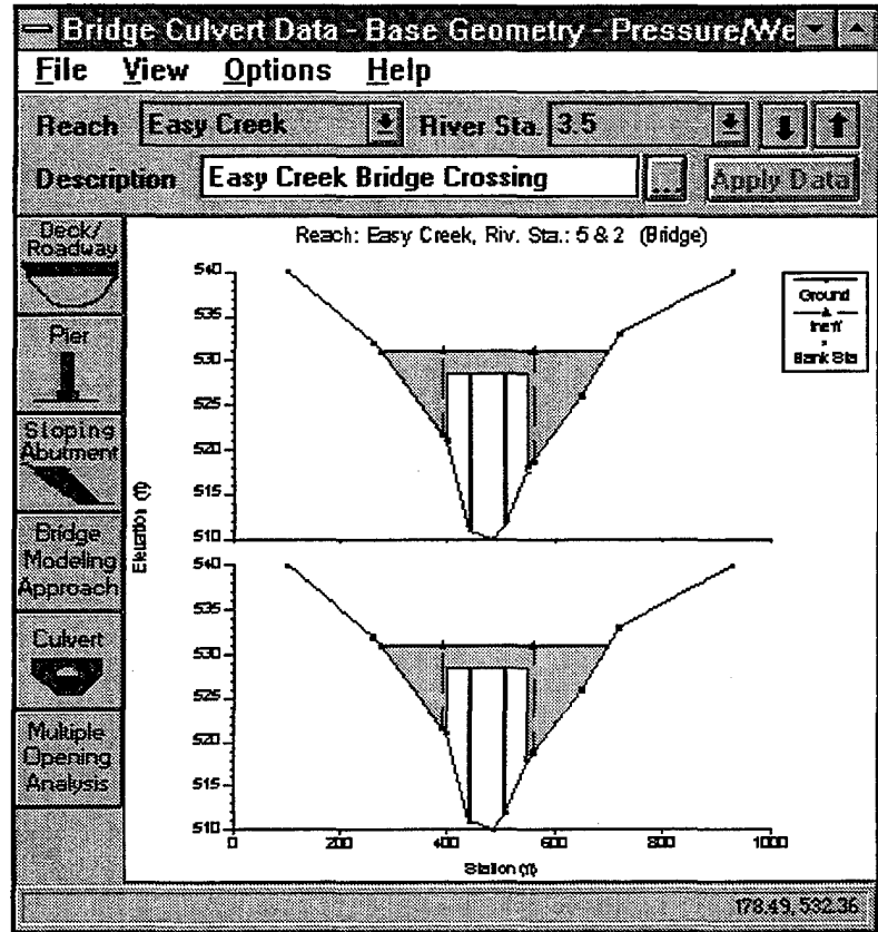
Figure 3. HEC-RAS Bridge Data Editor
