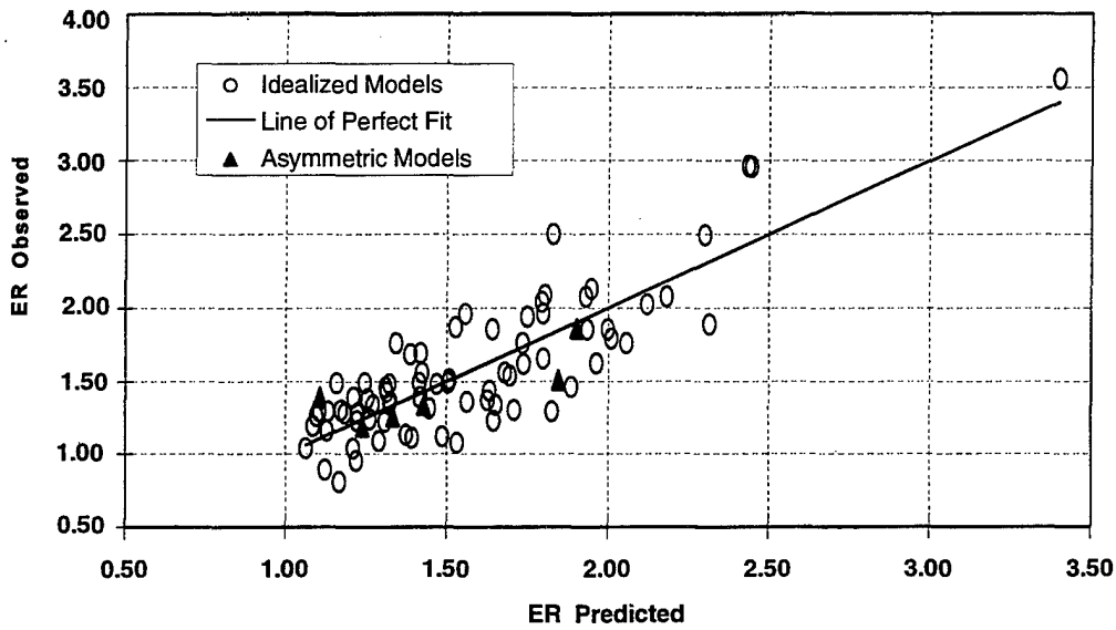
Figure 6. Goodness-of-Fit Plot for Expansion Ratio Regression Equation (Equation 2).
