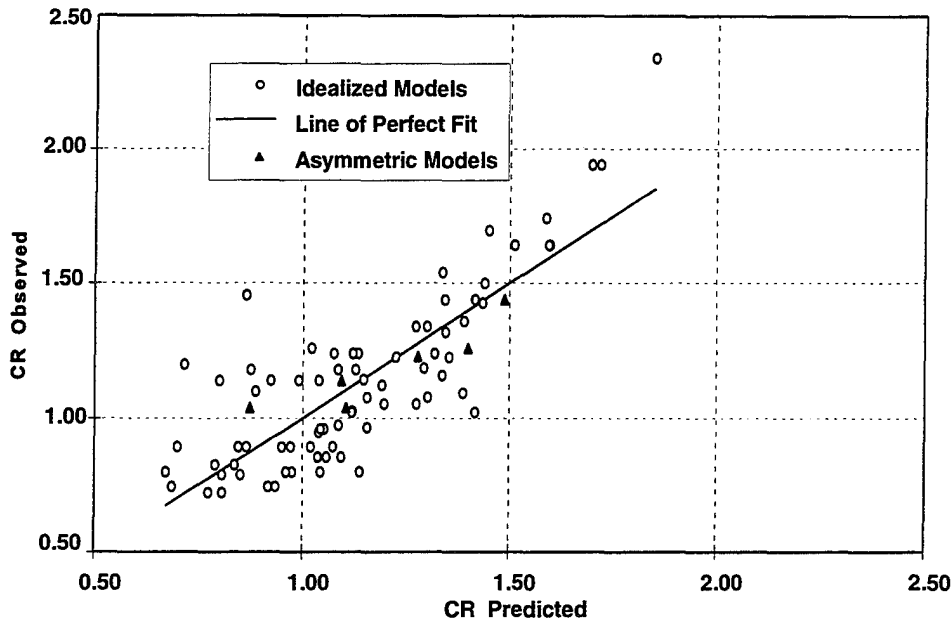
Figure 8. Goodness-of-Fit Plot for Contraction Ratio Regression Equation (Equation 4).
